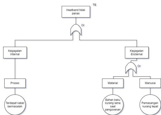
Gambar 4. Gambar FTA kegagalan band heater
